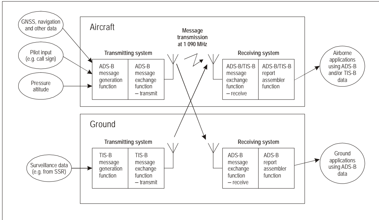
Figure 5-1. ADS-B/TIS-B system functional model
