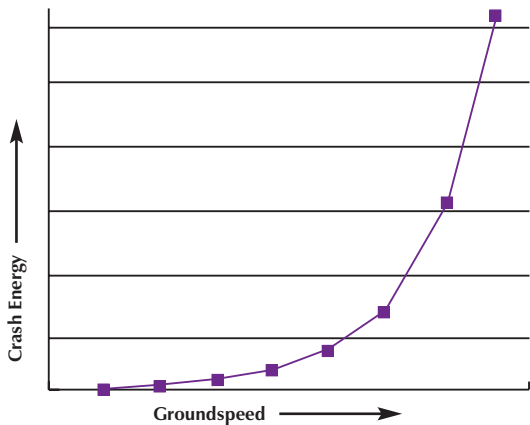
Energy increases with the square of speed. A 60-knot landing is only 50 percent faster than a 40-knot landing, but involves 125 percent more energy.
