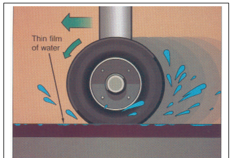
Figure 1a. Viscous hydroplaning (normal wet runway friction). A thin film of water acts like a lubricant. The microtexture of the runway surface (sandpaper-like roughness) breaks up the water film & greatly improves traction
